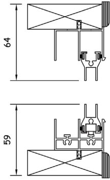
Cill Detail
